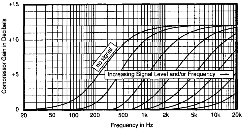
Fig. 6 High Freq. Sliding Band Compressor Characteristics
