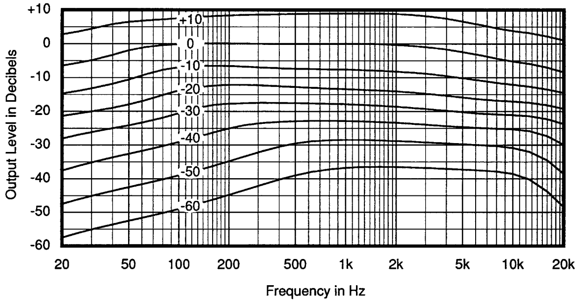
Fig. 16 S-Type Encoder Response versus Level and Frequency
