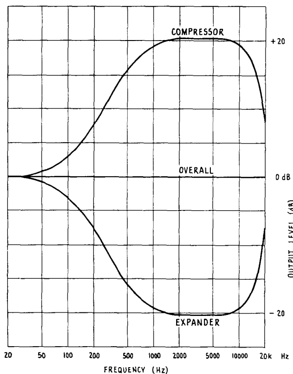
Fig. 17. Low-level (sub-threshold) frequency response of C-type compressor and expander.
