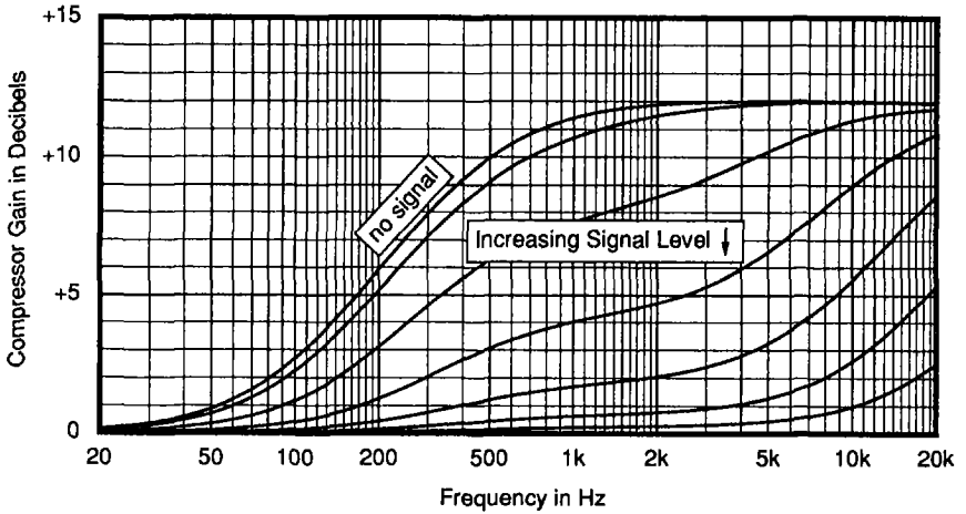
Fig. 8 Action Substitution Compressor Characteristics
