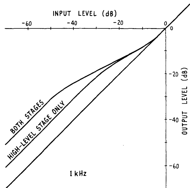
Fig. 14. Input-output transfer characteristic of C-type compressor at 1 kHz. High-level stage also shown.
