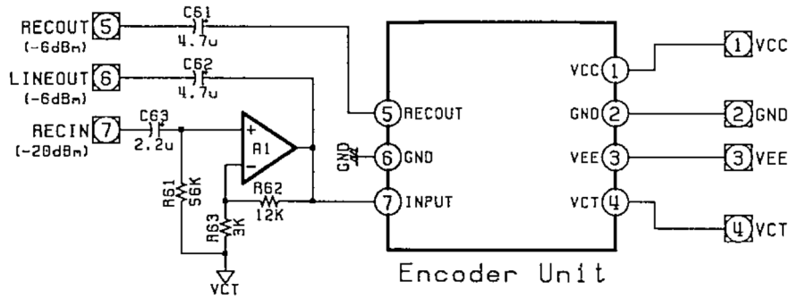
Fig. 2 Recording Processor
