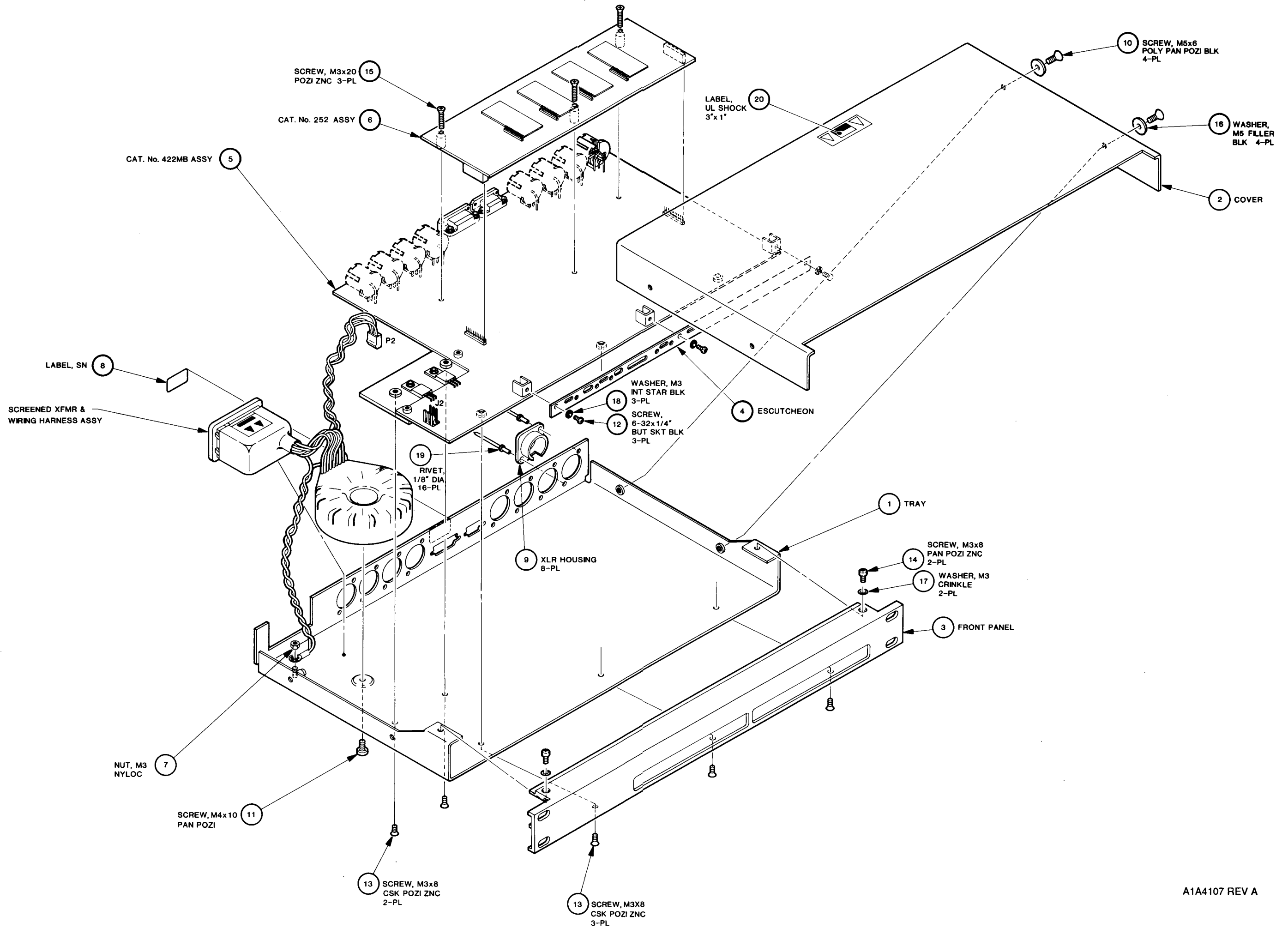
Figure 7.1 Model 422 tray assembly
