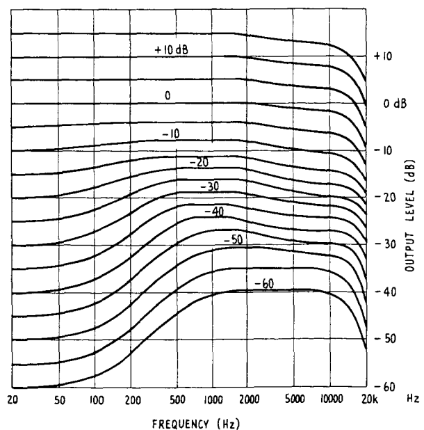
Fig. 15. C-type compression characteristics.
