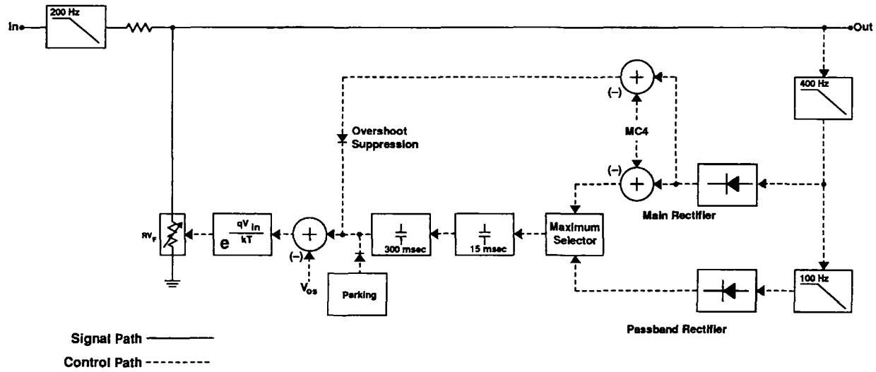
Fig. 14 Low Freq. Stage Block Diagram
