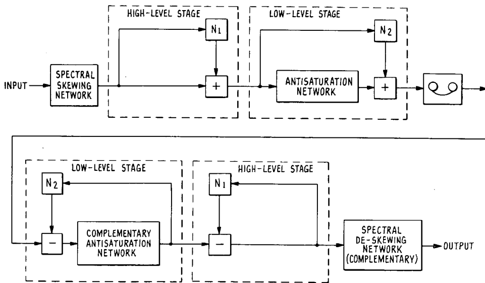
Fig. 10. Basic block diagram of C-type compressor and expander. N_1 and N_2 are the noise reduction networks.
