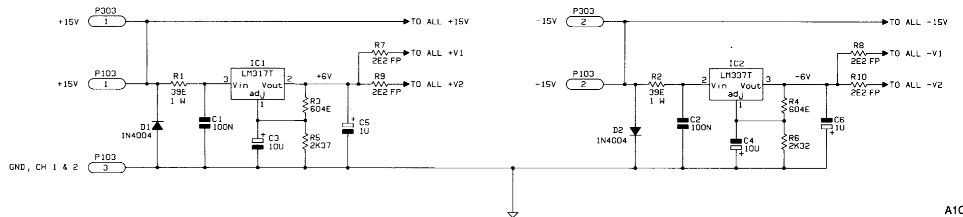
Figure 6.5 Cat. No. 252—S-type board
