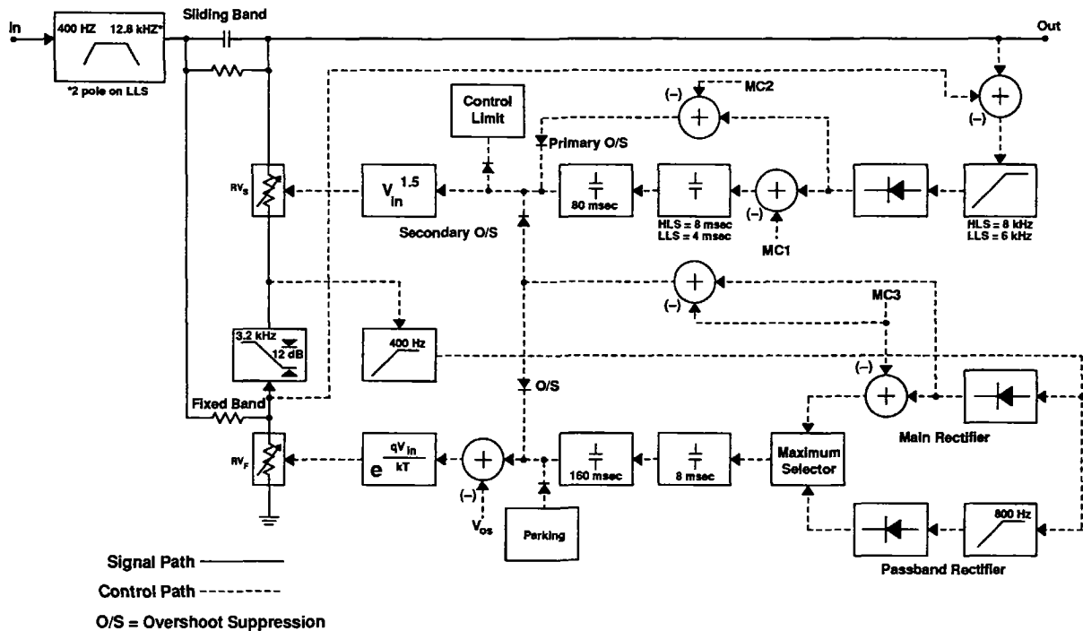
Fig. 13 High Freq. Stage Block Diagram
