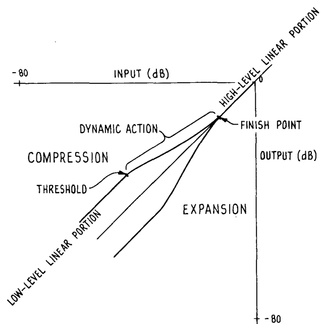
Fig. 1. Bilinear compression and expansion characteristics.
