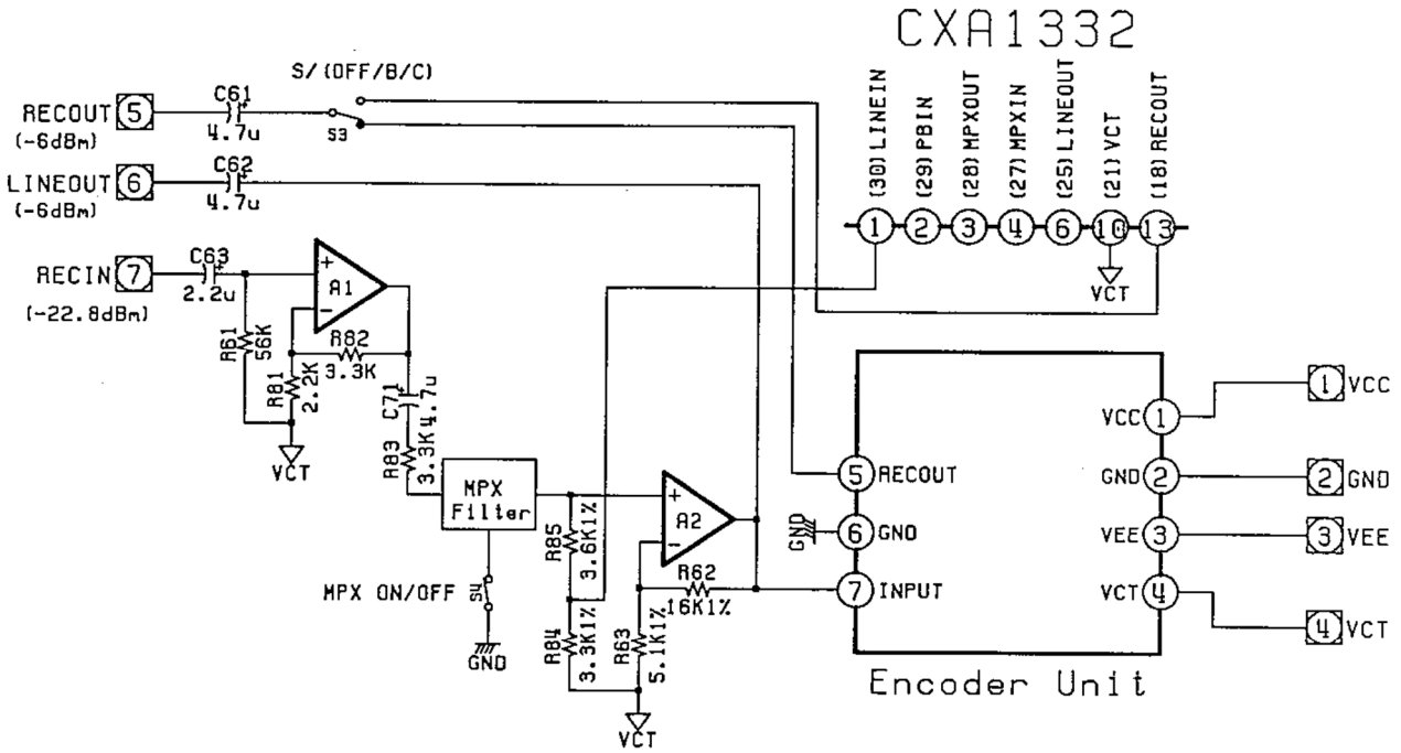
Fig. 5 Recording Processor With B/C type
