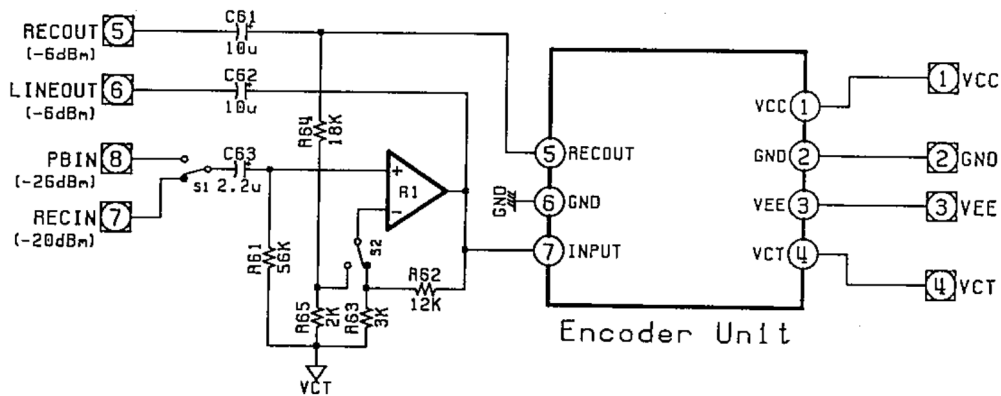
Fig. 4 Switchable Processor
