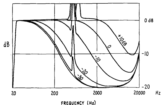
Fig. 20. Sliding band operation of expander with 500 Hz signal at the levels indicated ( -45 dB probe tone).
