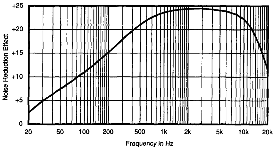
Fig.18 Maximum Noise Reduction Effect versus Frequency
