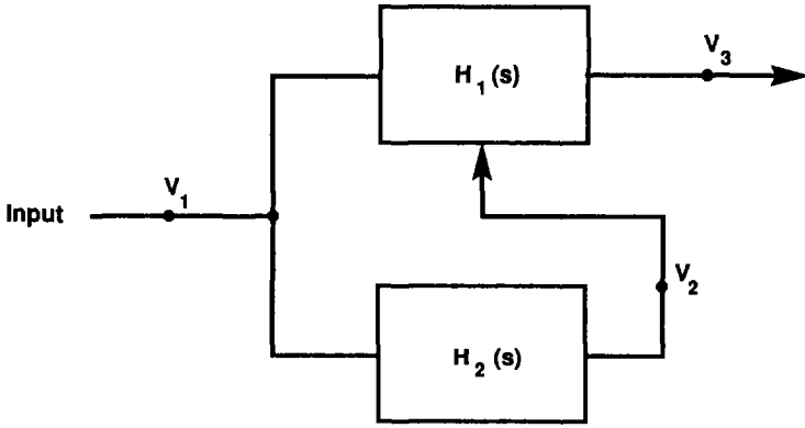
Fig. 7 The Action Substitution Configuration
