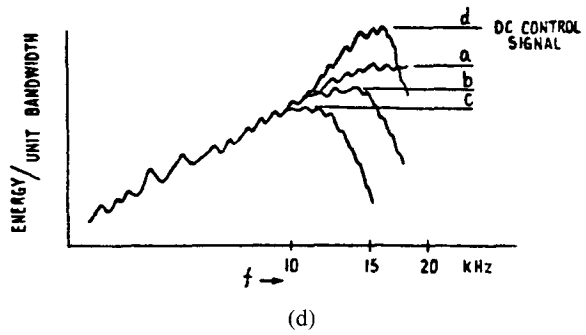
Fig. 6(d). The signal of (a) compressed and then sent through recorder channels a, b, c, d, resulting in the above signal distributions at the point of rectification in the expander; different dc control signals a, b, c, d are thereby produced.
