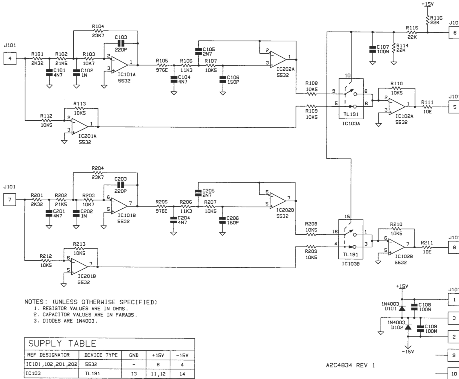
Figure 6.6a Cat.No.435A 20 kHz low-pass filter for S-type duplication.
