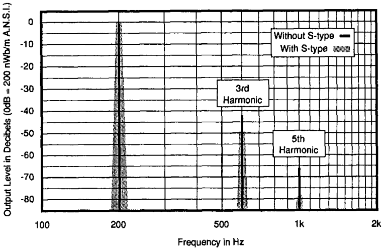
Fig. 21 Harmonic Distortion of 200 Hz Tone
