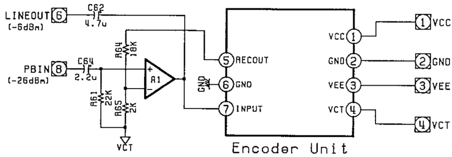
Fig. 3 Playback Processor
