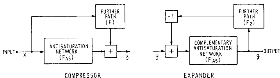
Fig. 9. Placement of antisaturation networks in main signal paths of compressor and expander.
