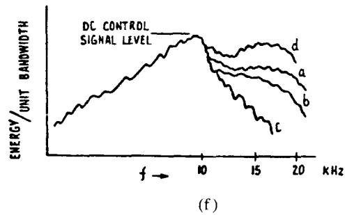
Fig. 6(f). As (d), but with spectral skewing treatment at the input of the compressor; the same dc control signal is produced in the expander with the four different recorder responses a, b, c, d.
