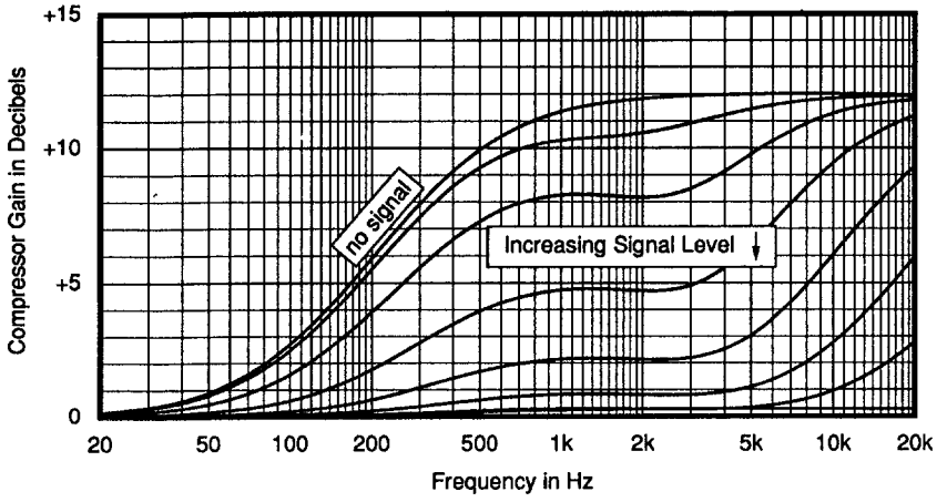
Fig. 9 S-type Action Substitution Compressor Characteristics
