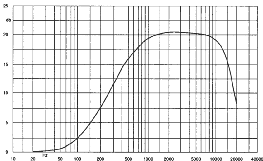
Figure 2.4 Low-level response of C-type encoder
