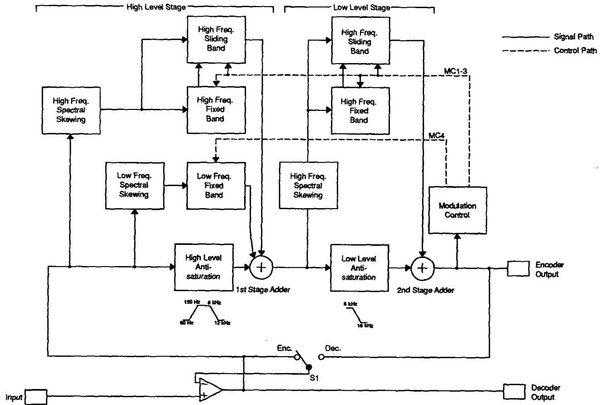
Fig. 12 S-type Processor Block Diagram
