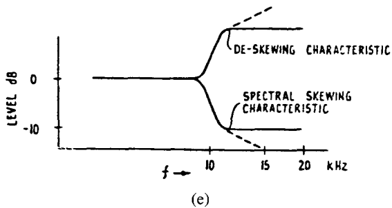
Fig. 6(e). Idealized spectral skewing characteristic.
