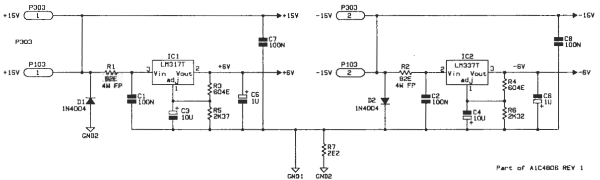
Figure 6.5a Cat.No.252A S-type board
