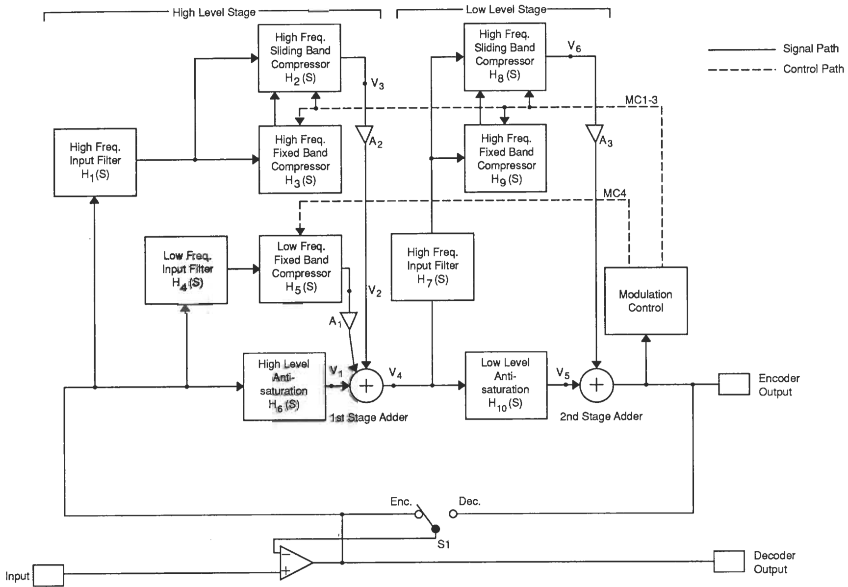
Figure 2.6 Block diagram of S-type encoder
