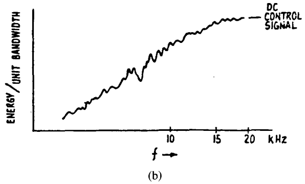
Fig. 6(b). The signal of (a) after control amplifier preemphasis in the compressor.
