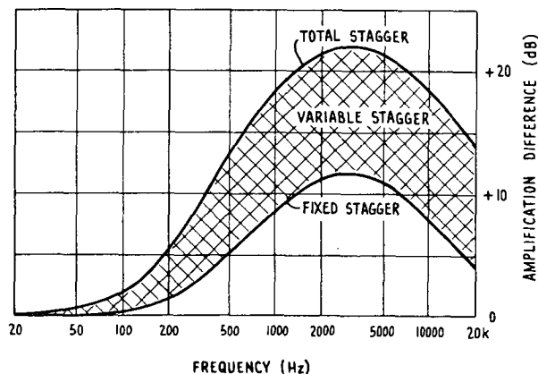
Fig. 13. Control-circuit amplification difference between high-level stage and low-level stage. The low-level stage has a fixed gain increase which is augmented by a variable increase caused by the signal-processing action of the high-level stage.
