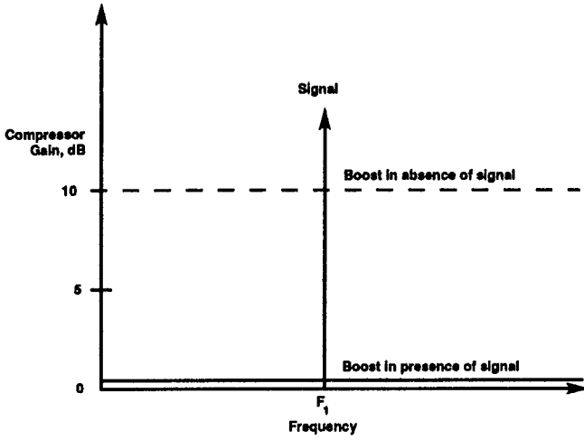
Fig. 1 Simple Compressor Action
