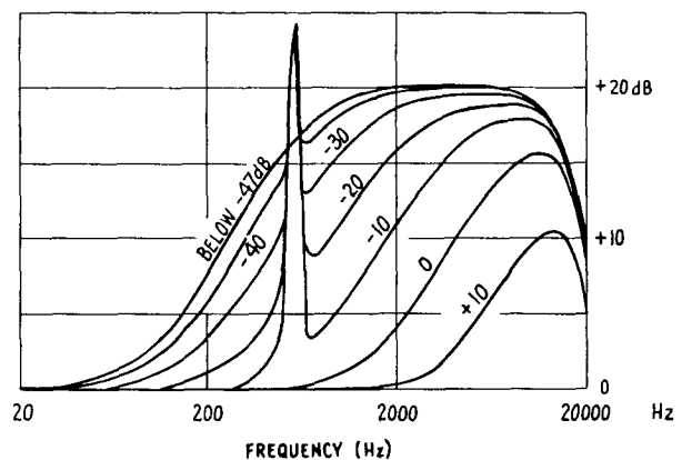
Fig. 19. Sliding band operation of C-type compressor with 500 Hz signals at the levels indicated ( -65 dB probe tone).
