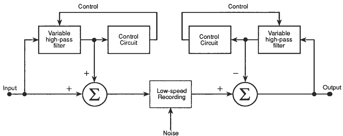
Figure 2.1 Block diagram of B-type noise reduction
