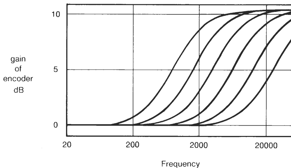
Figure 2.2 Family of response curves for B-type encoder
