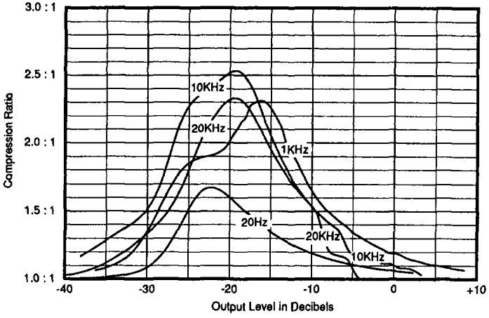
Fig. 17 Compression Ratio versus Output Level
