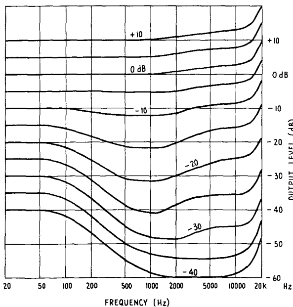
Fig. 16. C-type expansion characteristics.
