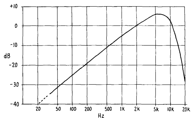
Fig. 5. CCIR noise-weighting characteristic (CCIR/ARM).
