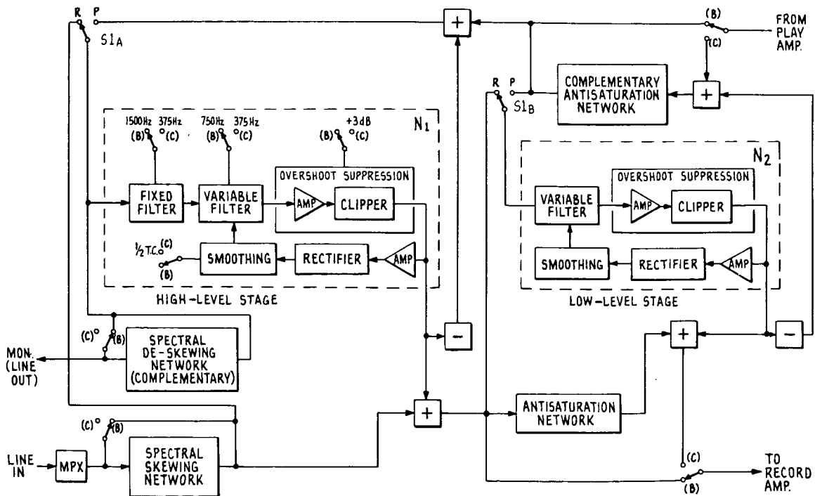
Fig. 11. Switchable record/play and B-type/C-type processor.
