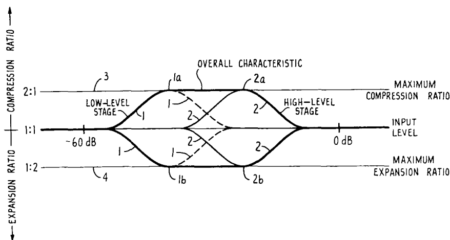
Fig. 3. Action-staggering principle.
