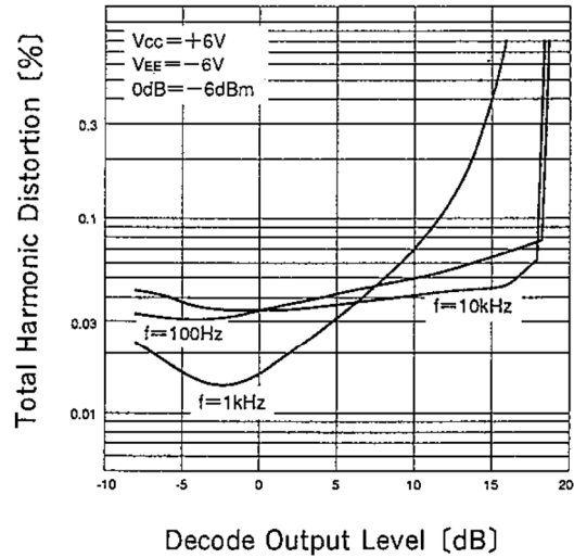
Decode THD Characteristics
