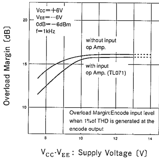
Overload Margin vs Supply Voltage
