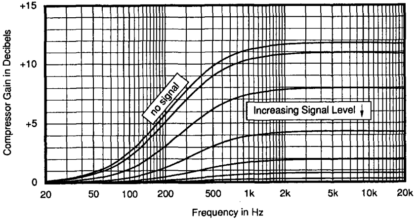
Fig. 5 Fixed Band Compressor Characteristics
