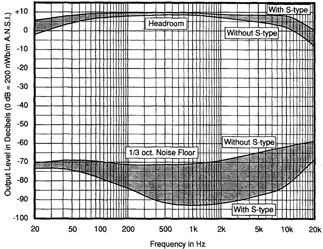
Fig. 22 Dynamic Range Improvement for Type IV Tape
