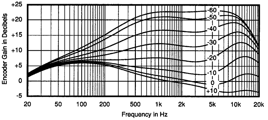
Fig. 19c Encoder Gain in the Presence of a 3 kHz Signal
