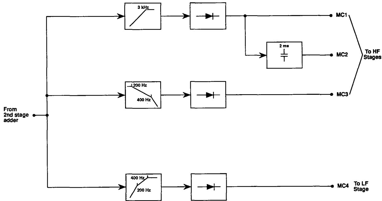
Fig. 15 Modulation Control Circuits Block Diagram
