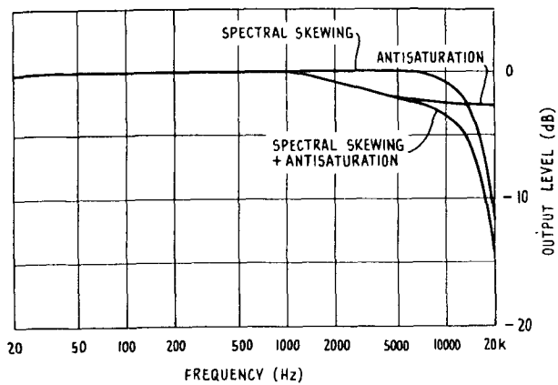
Fig. 7. Spectral skewing and antisaturation characteristics used in C-type system. Overall antisaturation effect is produced by combination of the two characteristics.
