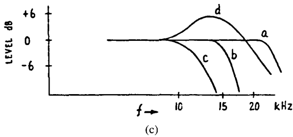
Fig. 6(c). Four different tape recorder frequency responses (a, b, c, d).
