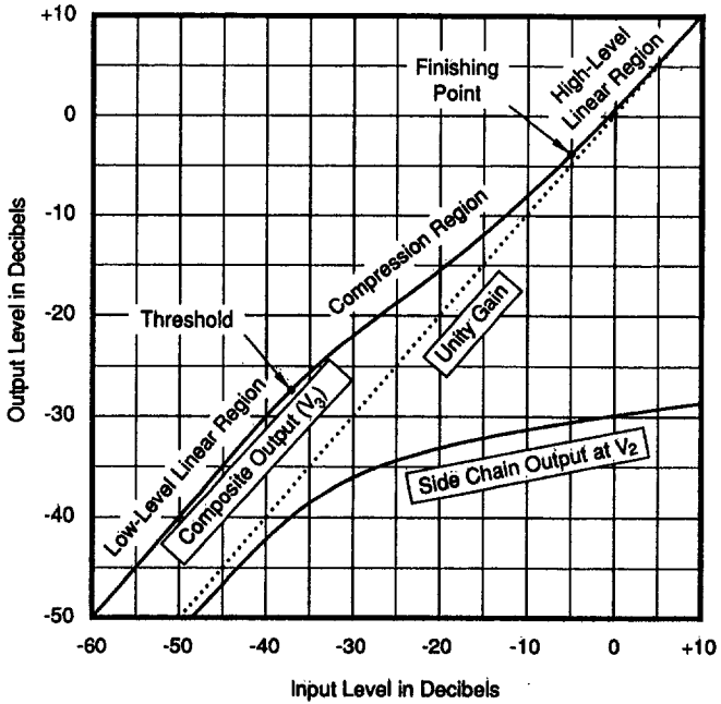
Fig. 4 Bilinear Compressor Characteristics
