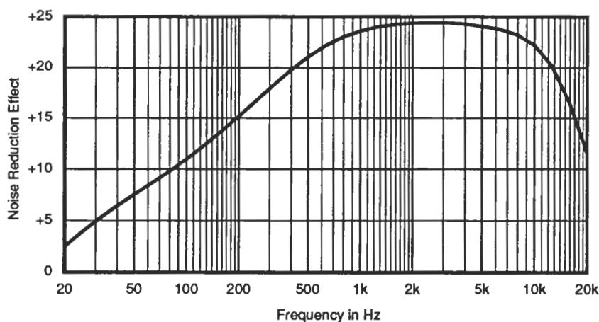
Figure 2.5 Low-level response of S-type encoder
