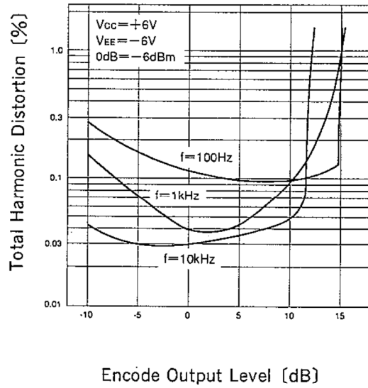
Encode THD Characteristics
