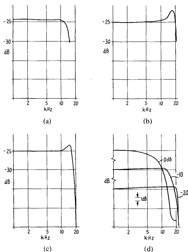
Fig. 8. Measured high-frequency responses of four typical cassette recorders.
