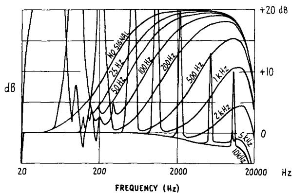
Fig. 18. Sliding band action of compressor in response to high-level (0 dB) signals at the frequencies shown (-65 dB probe tone).
