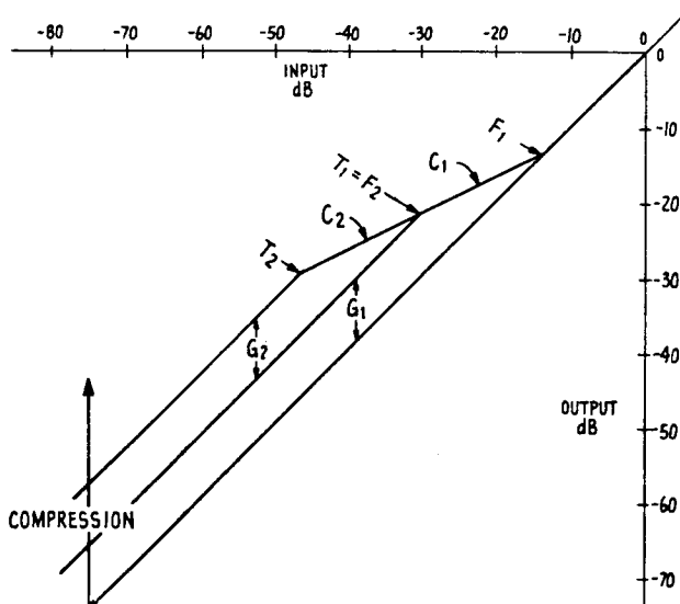
Fig. 4. Idealized construction to show parameter relationships (Eq. 1), C —compression ratio; T —threshold; F —finishing point; G —stage gain.
