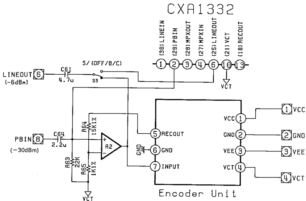
Fig. 6 Playback Processor with B/C type
