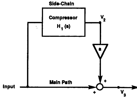
Fig. 3 Bilinear Compressor Block Diagram
