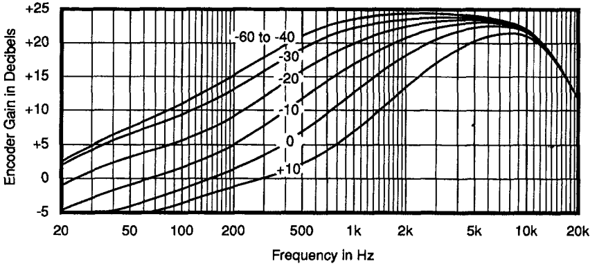
Fig. 19a Encoder Gain in the Presence of a 200 Hz Signal
