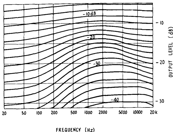
Fig. 12. Input-output characteristics of high-level stage only, without spectral skewing.
