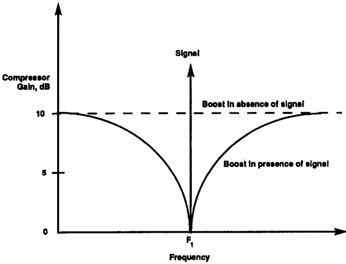
Fig. 2 Least Treatment Compressor Action
